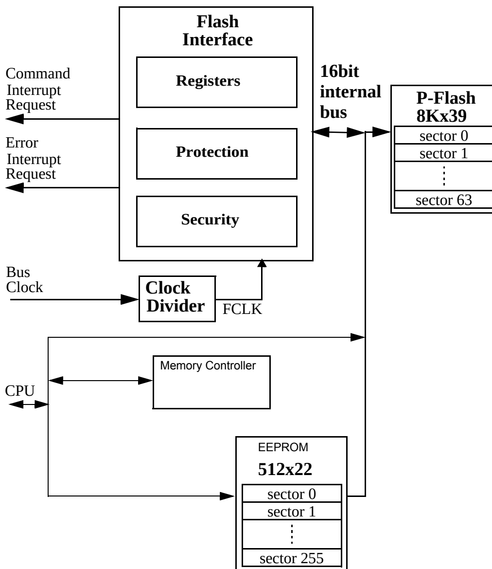
Figure 25-1. FTMRG32K1 Block Diagram
